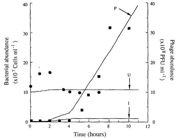
Fig. 1. Fit between simulated phage-host population dynamics and experimental data corresponding to Fig. 4A. Lines show expected dynamics of phage and bacteria based on the model. P; Phage population, U; uninfected bacterial population, I; infected bacterial population. Solid squares; phage 21/50 abundance, solid circles; bacterial abundance.
