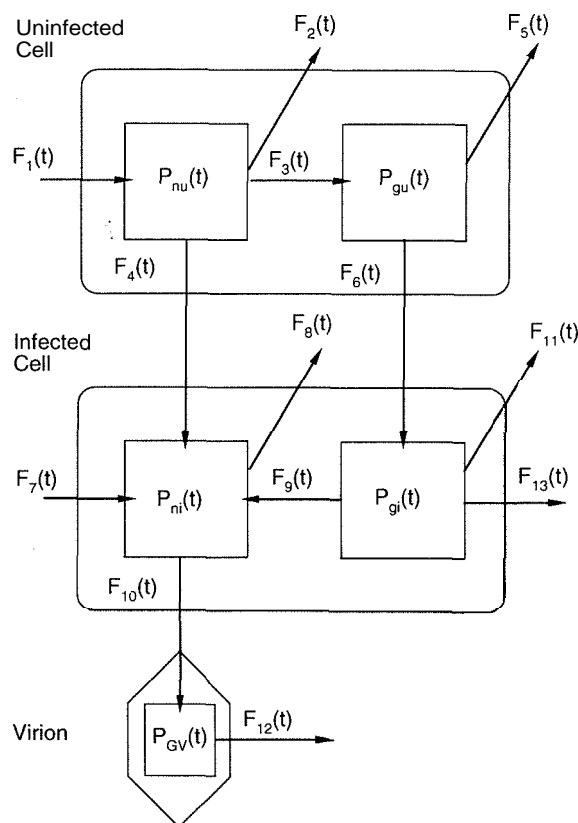
Fig. 2. Representation of ^{32}\text{P} -label in bacteria and phage nucleotide and nucleic acid pools. Balanced growth is assumed for uninfected bacteria. Nucleotides and nucleic acids in the infected bacteria are either excreted or synthesised (for nucleotides only), so that \gamma_{\text{nb}} and \gamma_{\text{gb}} remain constant. All pool concentrations in \text{nmole } ^{32}\text{P-nucleotide ml}^{-1} .
